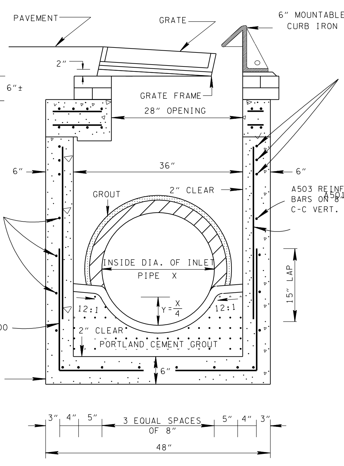
SECTION B-B
