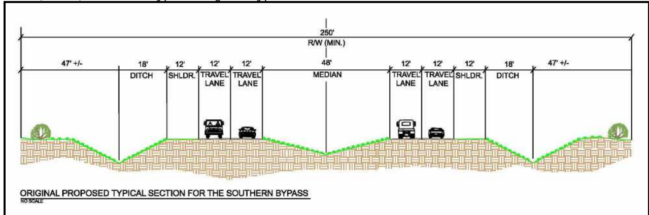
SR-15 (US-64) Southern Bypass Original Typical Section
