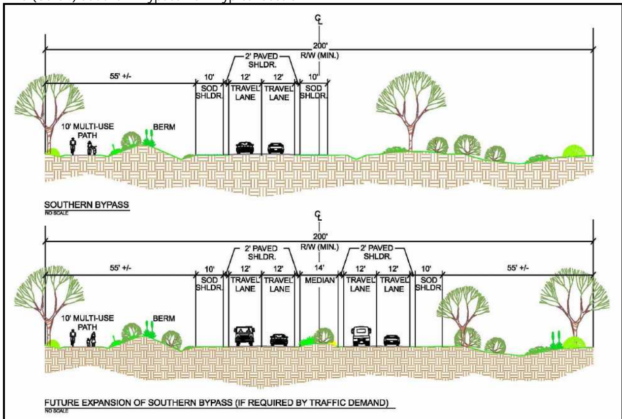
SR-15 (US-64) Southern Bypass New Typical Section
